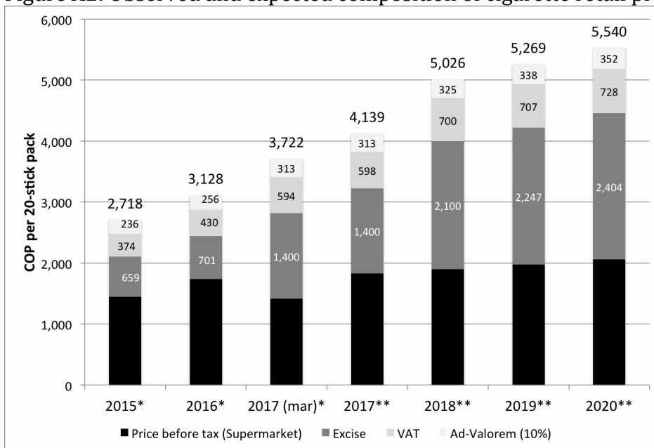
Figure A2: Observed and expected composition of cigarette retail prices in Colombia
