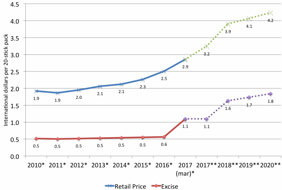
Figure A1: Cigarette retail prices and excise tax in Colombia
